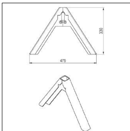
A-frame: CAT Communal
