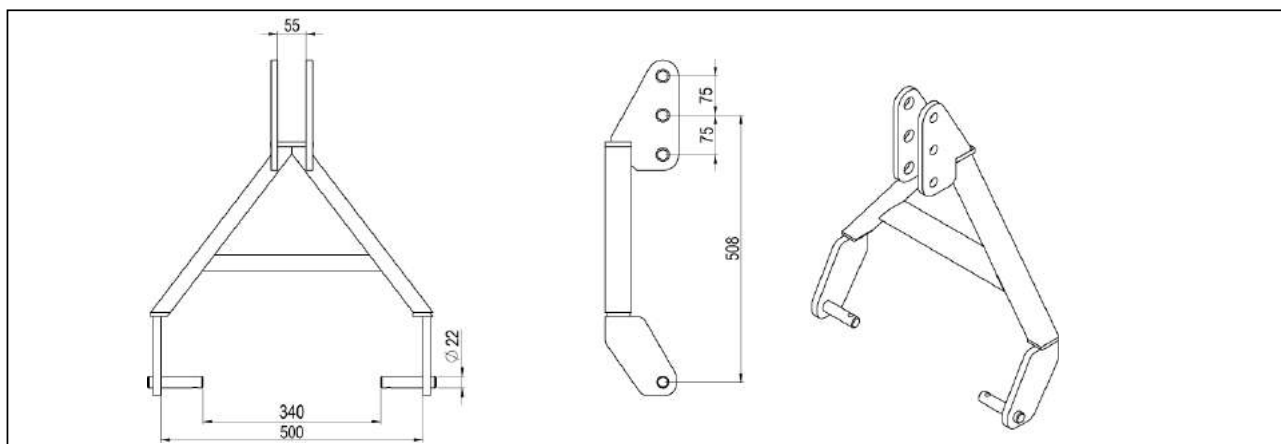
Three-point linkage: CAT I N
