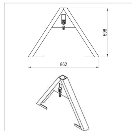
A-frame: CAT I
