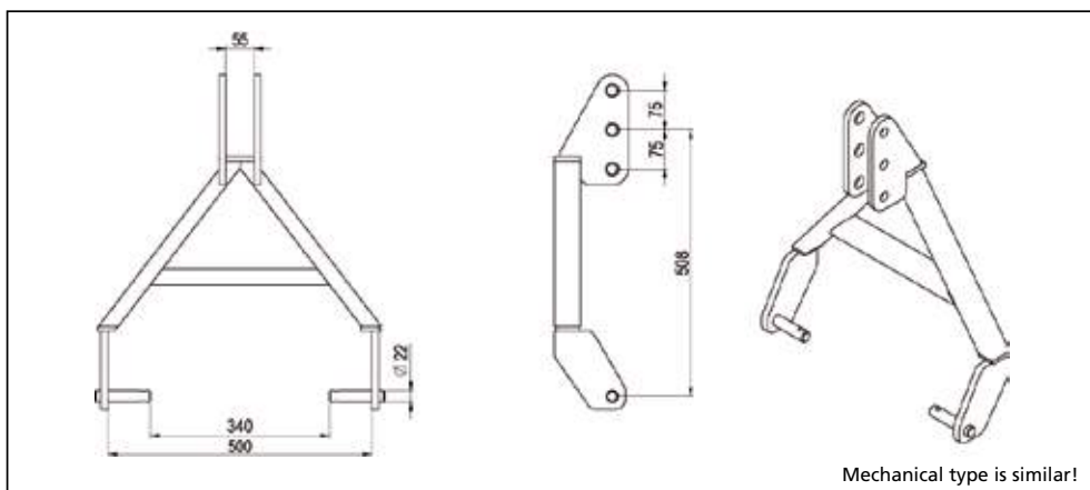
Three-point linkage: CAT I N
